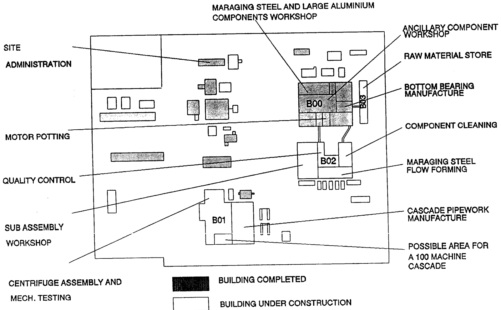
FIGURE 2. THE AL FURAT CENTRIFUGE PRODUCTION COMPLEX
